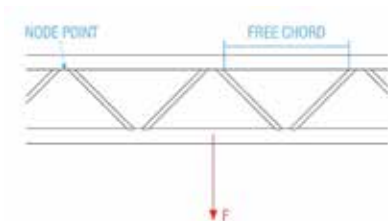
Load application at the free chord between two node points
