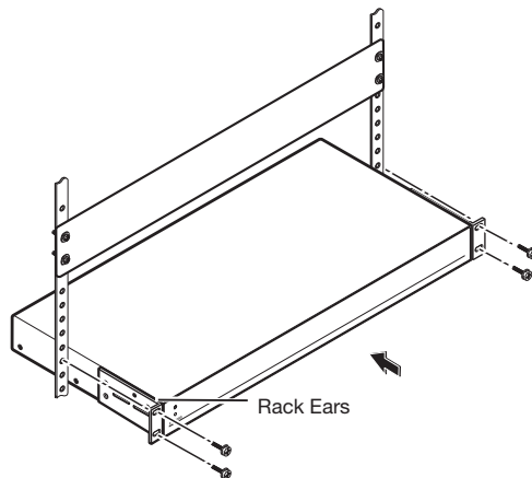
Figure 63. 1U Rack Mounting
