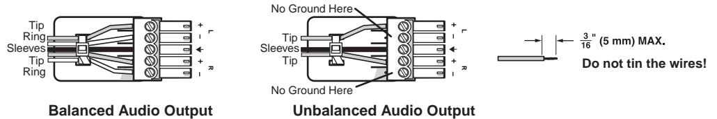
Figure 8. Audio Output Connector Wiring
