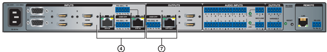
Figure 4. Rear Panel Connectors on IN1608 Models
