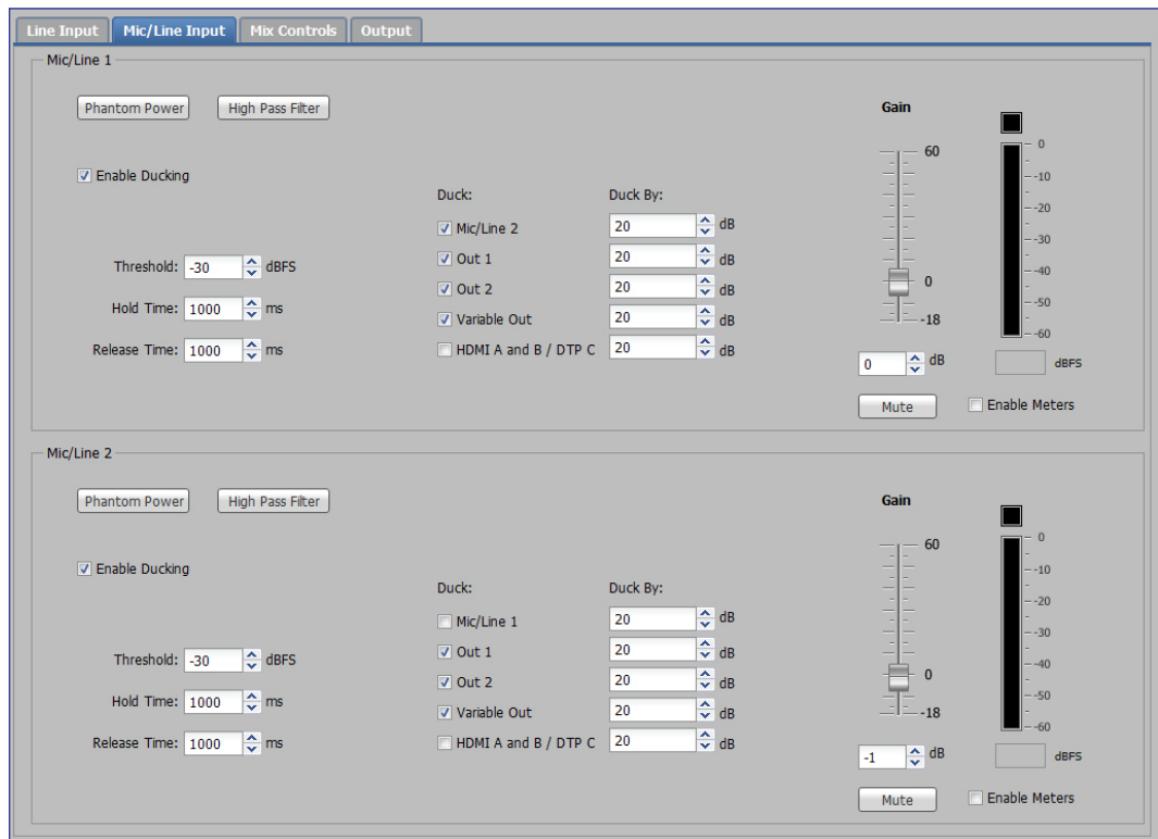
Figure 45. Mic/Line Input Tab with Ducking Enabled (IN1608)
