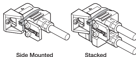
Figure 10. LockIt Bracket Mounting Options
