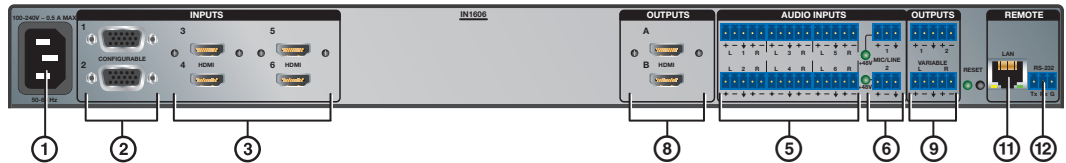
Figure 3. Shared Rear Panel Connectors
