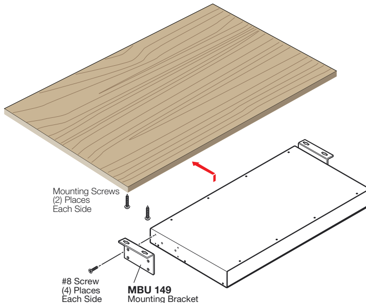
Figure 65. Under-Desk Mounting
