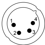
Figure 35: XLR-4 male
