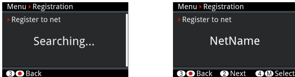
Figure 18: Net searching
