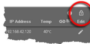
Figure 86: Login
